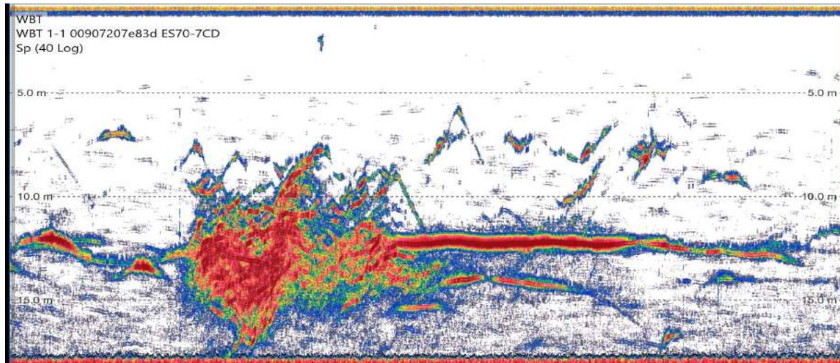
Figure 10-6. Example echogram from a bottom mounted split-beam echosounder (70 kHz Simrad EK80) illustrating a school of white grunt ( Haemulon plumieri ) interacting with a barracuda ( Sphyræna barracuda ) near the Aquarius reef base in the Florida Keys.
