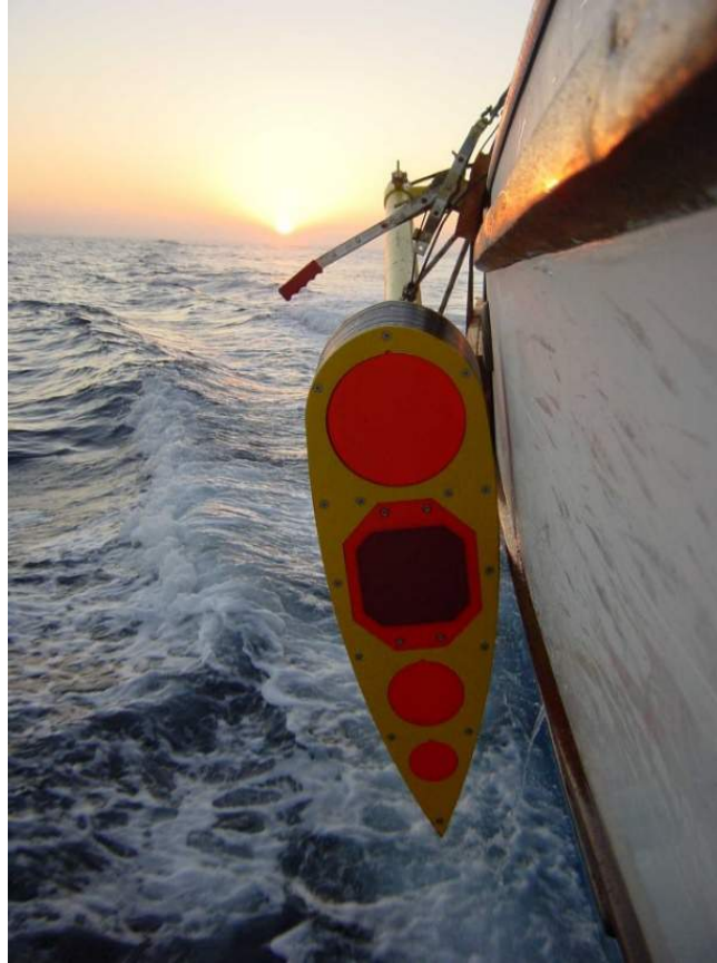
Figure 4-3. A portable four-frequency transducer array (top-bottom: Simrad ES70-7C, ES38-12, ES120-7C, and ES200-7C). To deploy, the array is lowered into the water such that the transducers are > 1-m deep and projecting downward, and stabilizing lines are ratcheted tightly, fore and aft.
