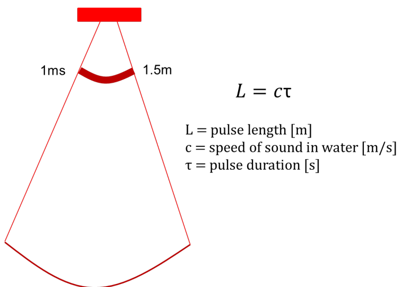
Figure 6-8. Illustration of the acoustic beam and sound pulse with duration of 1 ms and pulse length of 1.5 m.
