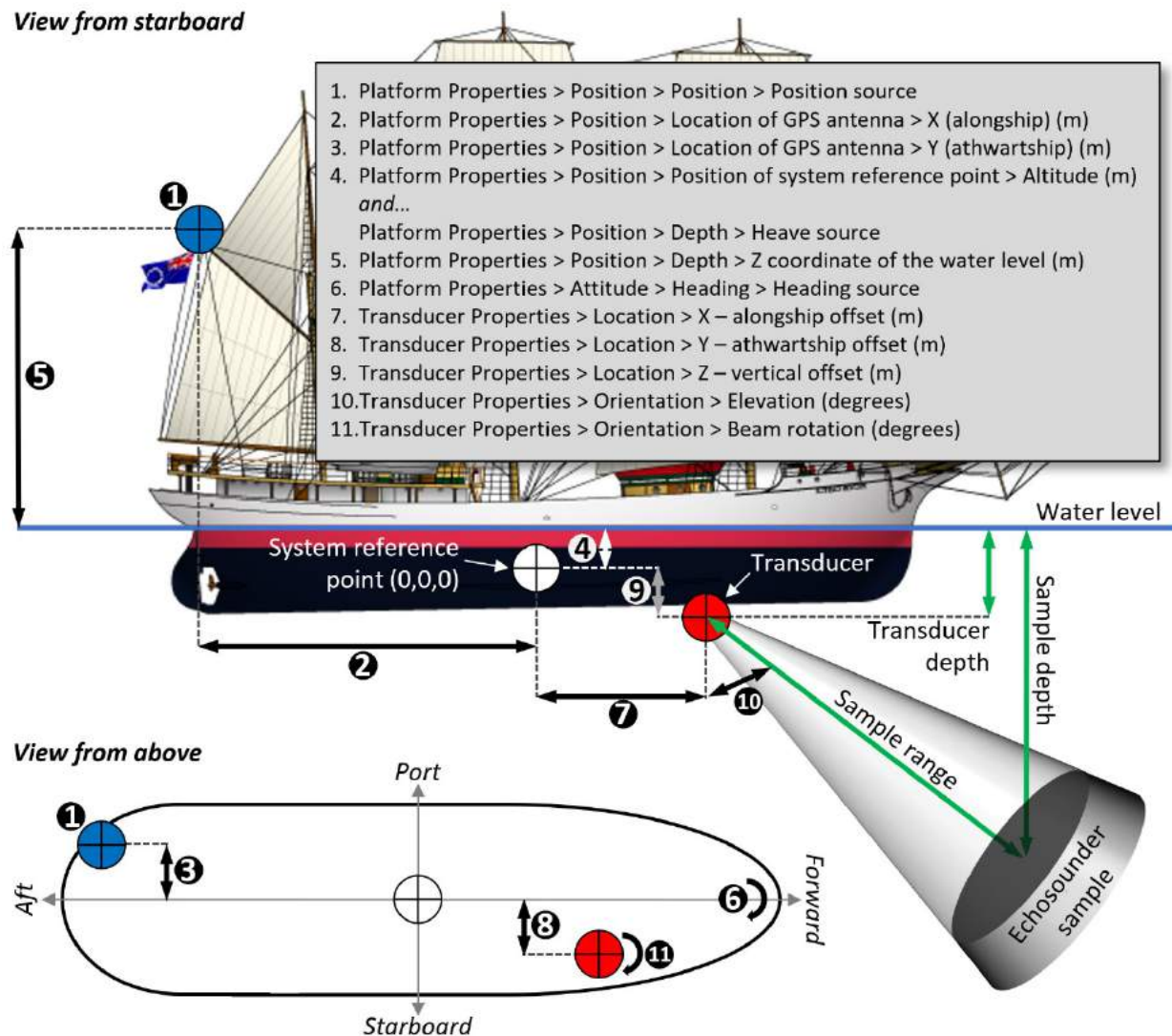
Figure 7-3. Factors contributing to the calculation of latitude, longitude, time and depth for a given echosounder sample. In this example the echosounder platform is a mobile surface vessel, but the principles can be extended to other mobile and stationary platforms such as towed bodies, autonomous underwater vehicles, probes, moorings and landers. The text box represents Echoview 8 settings.
